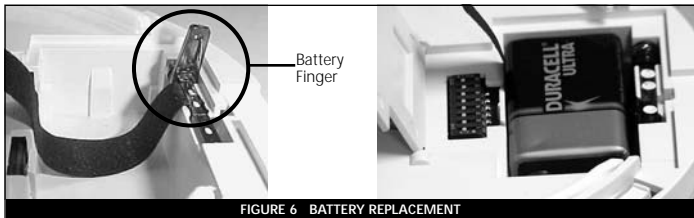
FIGURE 6 BATTERY REPLACEMENT
