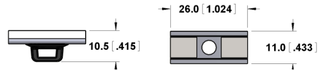
Magnetic Zip Tie Holder- Rectangle RES-62422-B
