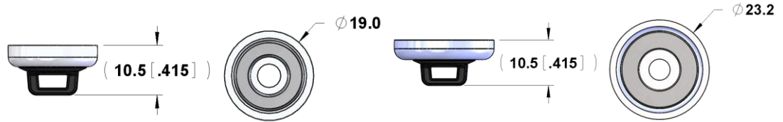
Large Magnetic Zip Tie Holder RES-62416-W / RES-62416-B
