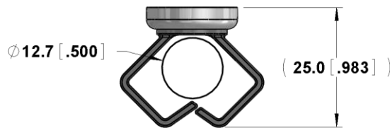
Medium Magnetic Wire Holder RES-62413-B / RES-62413-B
