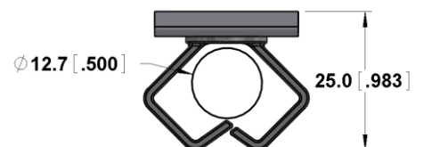
Medium Magnetic Wire Holder- Rectangle RES-62424-B
