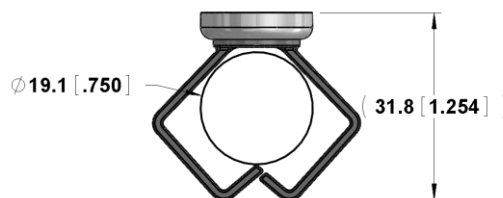
Large Magnetic Wire Holder RES-62415-W / RES-62415-B
