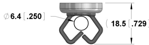
Small Magnetic Wire Holder RES-62401-W / RES-62401-B
