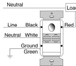
DW-100 and DW-100-347 Wiring
