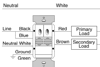
DW-200 Bi-Level Wiring
