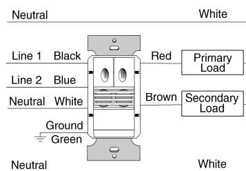
DW-200 Dual Circuit Wiring
